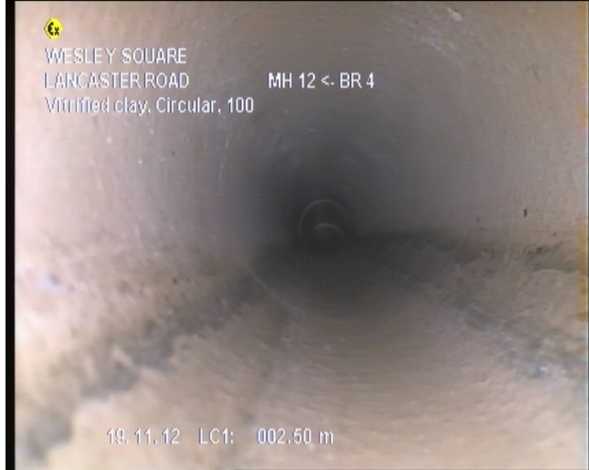
Photo: 23_5A 2.5m, Circumferential Crack, from 12 to 12 o'clock
