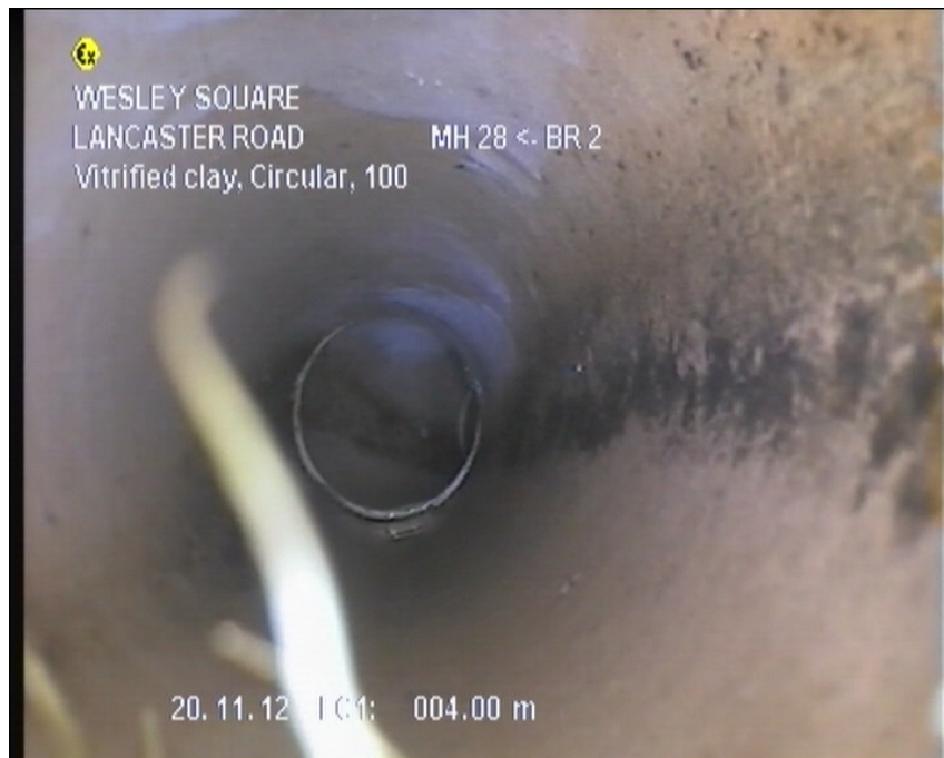
Photo: 81_7A 4m, Circumferential Crack, from 12 to 12 o'clock
