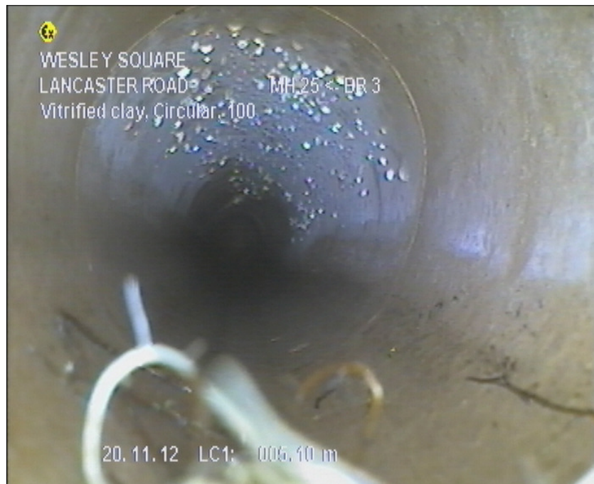
Photo: 485_7a 5.1m, Circumferential Crack, from 12 to 12 o'clock
