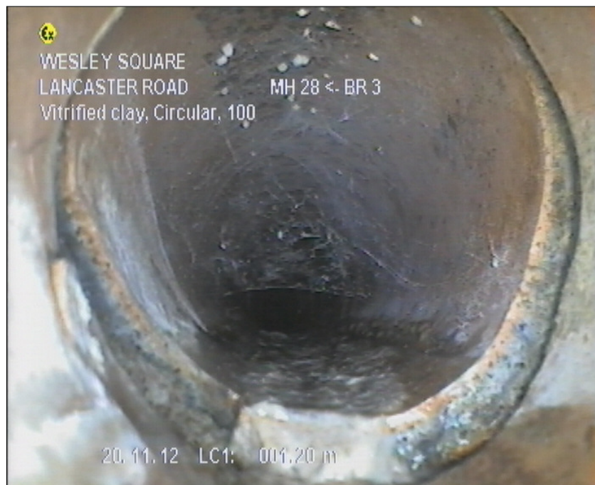
Photo: 572_6a 1.2m, Joint displaced. Medium
